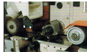
雙主軸設計，可搭配圓棒刀、 花棒刀及成型刀...等。 Two spindle suit for smooth dowel cutter fluted dowel cutter and profile cutter...etc.
