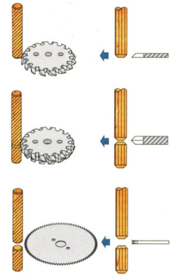
木樁倒角及切斷 Dowel chamfering & cutting
